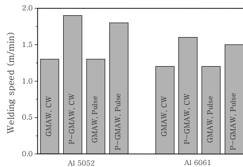
Fig. 2 Maximum welding speed to achieve full penetration for each process
