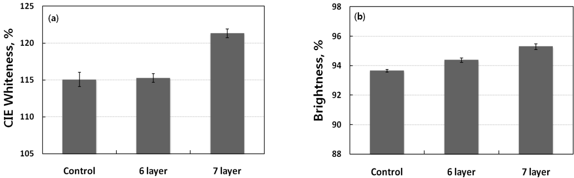
Fig. 1. Effect of LbL multilayering of C-starch and PSS on whiteness (a) and brightness (b) of paper.
