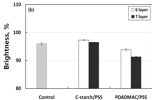
Fig. 5. Whiteness (a) and brightness (b) of surface sized paper made from pulp fibers with LbL multilayering of C-starch/PSS and poly-DADMAC/PSS.
