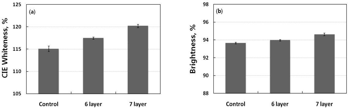
Fig. 2. Effect of LbL multilayering of poly-DADMAC and PSS on whiteness (a) and brightness (b) of paper.
