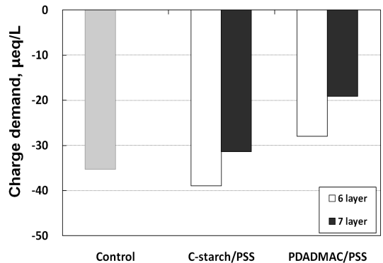
Fig. 3. Charge demand of the filtrate after interaction between FWA and pulp fibers.
