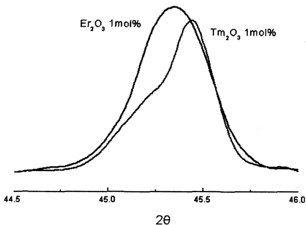
Fig. 5. Variation in XRD peaks in the 2θ range from 44.5 to 46, covering (002) and (200) peaks of BaTiO 3 specimens doped with Tm 2 O 3 and Er 2 O 3 .
