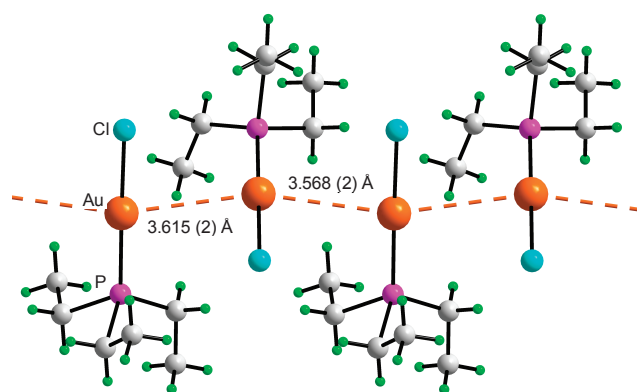
Figure 6. Supramolecular aggregation leading to a zigzag chain mediated by aurophilic ( \text{Au}\cdots\text{Au} ) interactions in the crystal structure of \text{Et}_3\text{PAuCl} , after ref. 12.
