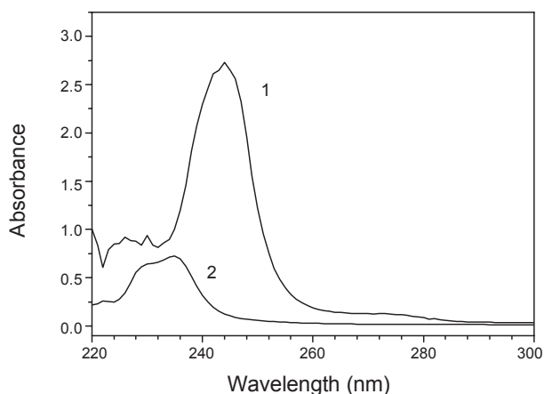
Figure 1. Absorption spectra of Et 3 P (1, 0.10 M) and Et 3 PAuCl (2, 3.0 × 10 -4 M) in THF.
