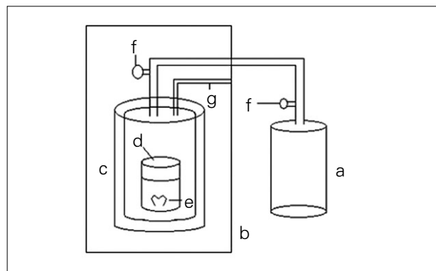
Figure 1. Schematic diagram of program freezer with pressure vessel.
