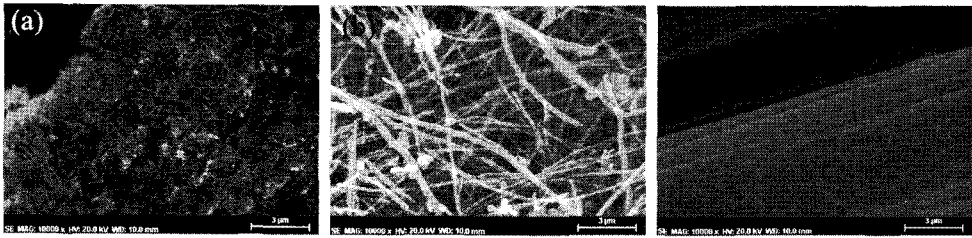
Fig. 1 SEM images of (a) CNT, (b) CNF, and (c) carbon fiber.
