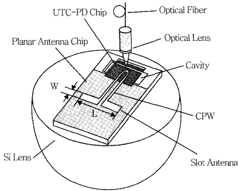
(그림 10) Conceptual Diagram of a MMW Photonic Transmitter[13]
