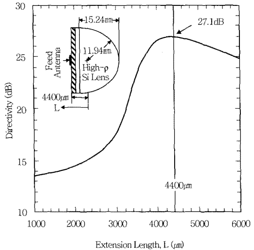
(그림 7) CPW-fed Slot-Ring Antenna and Directivity vs Extended Hemispherical Lens [10]
