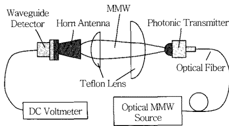
(그림 11) Photonic Transmitter and Output Power Measurement Test Setup[13]
