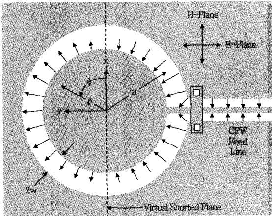
(그림 7) CPW-fed Slot-Ring Antenna and Directivity vs Extended Hemispherical Lens [10]
