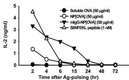
Figure 3. Time-kinetics for the cross-presentation of OVA peptides. DCs were incubated with soluble OVA (50 \mu g/ml), OVA-loaded NPs (50 \mu g/ml), IgG-opsonized OVA-loaded NPs (50 \mu g/ml), or 1 nM synthetic OVA peptide (SIINFEKL) for 2 h. The DCs were then washed with PBS, and were cultured in a medium containing 10% fetal bovine serum. At the indicated time points, the DCs were fixed with paraformaldehyde, and the amounts of OVA peptides presented on MHC class I molecules were assessed by a LacZ T cell activation assay using OVA specific CD8 T cell hybridomas, B3Z cells.
