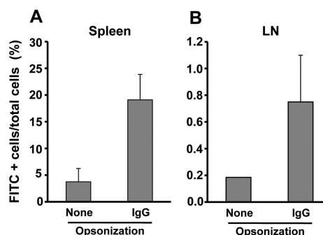
Figure 4. The uptake and biodistribution of NPs injected into the mouse peritoneum. C57BL/6 mice were injected i.p. with 100 \mu g of NPs containing both OVA and FITC. Mice were sacrificed 2 h later, and mononuclear cell suspensions were prepared from the spleens (A) and lymph nodes (popliteal, inguinal, mesenteric, and axillary) (B). The single cell suspensions were fixed with paraformaldehyde and analyzed for FITC-positive cells by flow cytometry.
