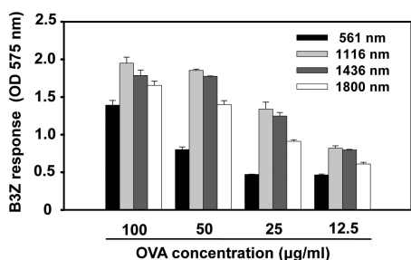
Figure 2. Effects of the size of NPs on the cross-presentation. DCs were incubated with NPs with different mean sizes for 2 h, washed with PBS, fixed with paraformaldehyde, and the amounts of OVA peptides presented on MHC class I molecules were assessed by a LacZ T cell activation assay using OVA specific CD8 T cell hybridomas, B3Z cells.
