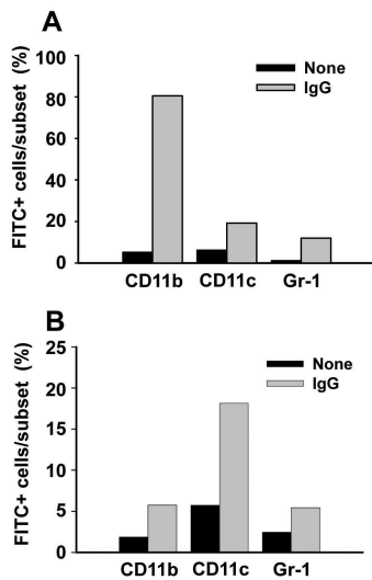
Figure 5. Cell type analysis for the FITC-positive cells in the spleen and lymph nodes. C57BL/6 mice were injected i.p. with 100 \mu g of NPs containing both OVA and FITC. The mice were sacrificed 2 h later, and mononuclear cell suspensions were prepared from the spleens (A) and lymph nodes (B), stained with phycoerythrin-labeled anti-mouse CD11b, CD11c, or Gr-1 monoclonal antibodies, and analyzed for FITC-positive cells by flow cytometry.
