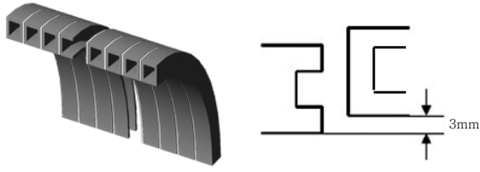
Fig. 2 Cross-section shape of PE double wall pipe: case 2
