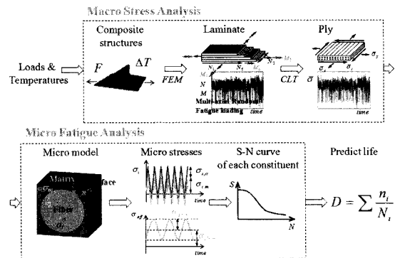
Fig. 1 MMF based fatigue life prediction procedure for composite structures.
