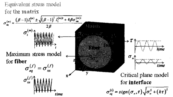
Fig. 4 MMF based fatigue models.
