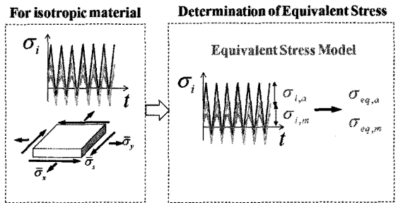
Fig. 5 Equivalent stress model for the multi-axial fatigue loading.
