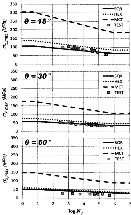
Fig. 8 Fatigue life prediction of the off-axis unidirectional laminae.
