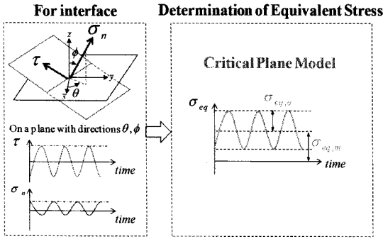
Fig. 6 Critical plane model for the interfacial fatigue.
