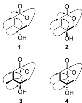
Figure 2. Key ^1\text{H} - ^1\text{H} COSY ( \leftrightarrow ) and HMBC ( \rightarrow ) correlations of 1-4 .
