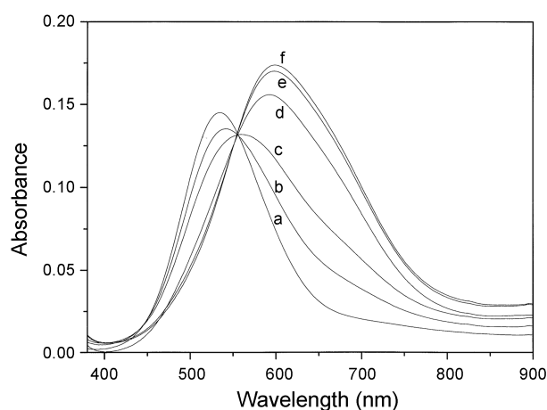
Figure 2. Visible absorption spectra of [\text{Cu}(\text{HL}^3)](\text{ClO}_4)_2 ( 1.0 \times 10^{-3} \text{ M} ) measured in NaOH water-acetonitrile (1:1) solutions at 25 °C; pH 7.0 (a), 11.4 (b), 12.0 (c), 12.7 (d), [\text{NaOH}] = 0.05 \text{ M} (e), and [\text{NaOH}] = 0.1 \text{ M} (f). The spectrum measured in 0.1 M \text{HClO}_4 solution is similar to curve a.
