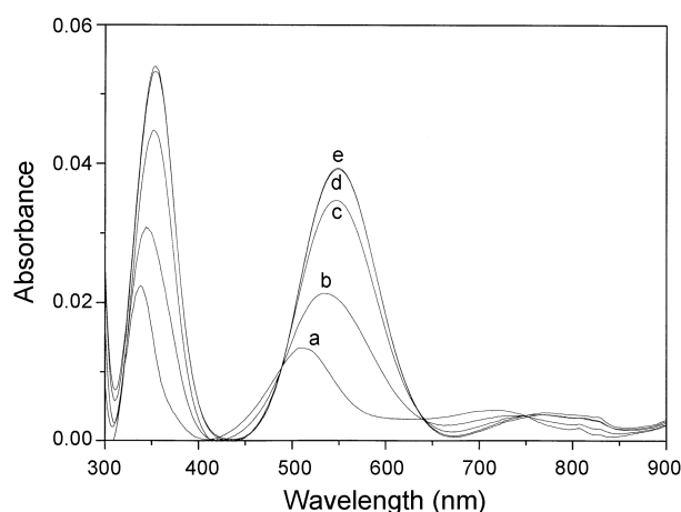
Figure 1. Visible absorption spectra of [\text{Ni}(\text{HL}^3)(\text{H}_2\text{O})](\text{ClO}_4)_2 ( 2.0 \times 10^{-3} \text{ M} ) measured in NaOH water-acetonitrile (1:1) solutions at 25 °C; pH 6.6 (a), 10.4 (b), 11.1 (c), 12.2 (d), and 12.7 (e). The spectra measured in 0.1 M \text{HClO}_4 and 0.1 M NaOH solutions are similar to curves a and e, respectively.
