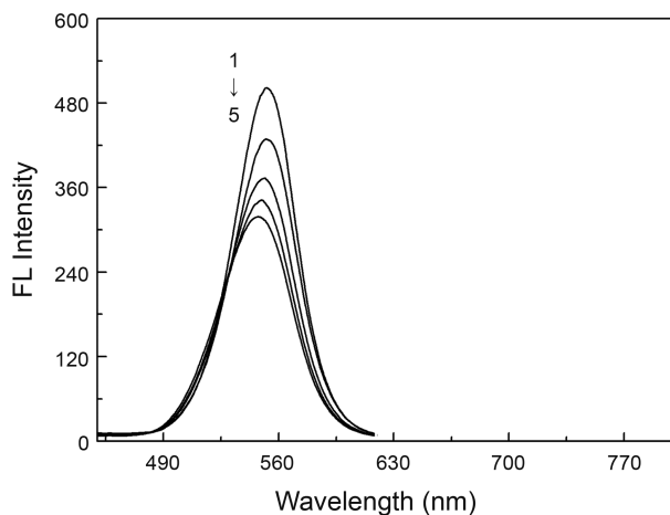
Figure 4. Effect of the temperature on fluorescence intensity of CdTe QDs, from 1 to 5: 20, 24, 28, 32, 36 °C.
