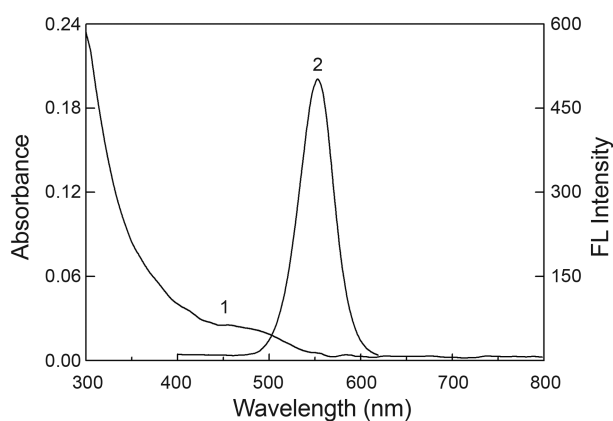
Figure 1. Absorption spectra (1) and fluorescence spectra (2, excited at 350 nm) of CdTe QDs.
