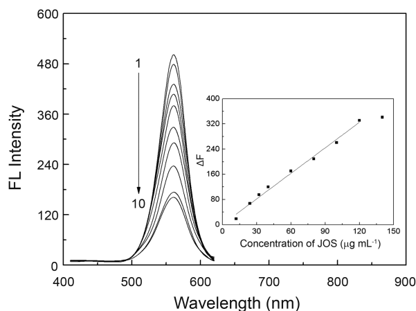
Figure 5. Fluorescence emission spectra of CdTe QDs in the absence and presence of different concentration of JOS: 0.0, 12.0, 24.0, 32.0, 40.0, 60.0, 80.0, 100.0, 120.0 and 140.0 \mu\text{g mL}^{-1} from 1 to 10.
