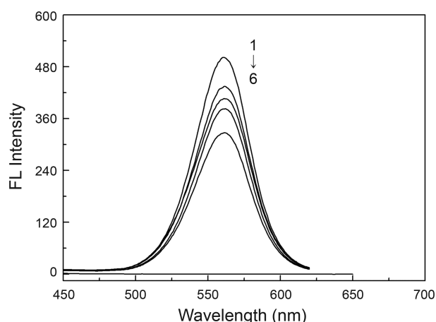
Figure 2. Fluorescence emission spectra of CdTe QDs in the absence and presence of different concentrations of JOS. Concentration of CdTe QDs from (1) to (5): 0.2 mmol L -1 , (6): 0 mmol L -1 ; JOS from (1) to (6): 0, 24, 32, 40, 60, 40 \mu\text{g mL}^{-1} .
