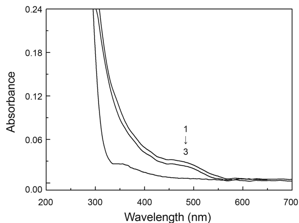
Figure 3. Absorption spectra of CdTe QDs in the presence of JOS (1), CdTe QDs (2), JOS (3).
