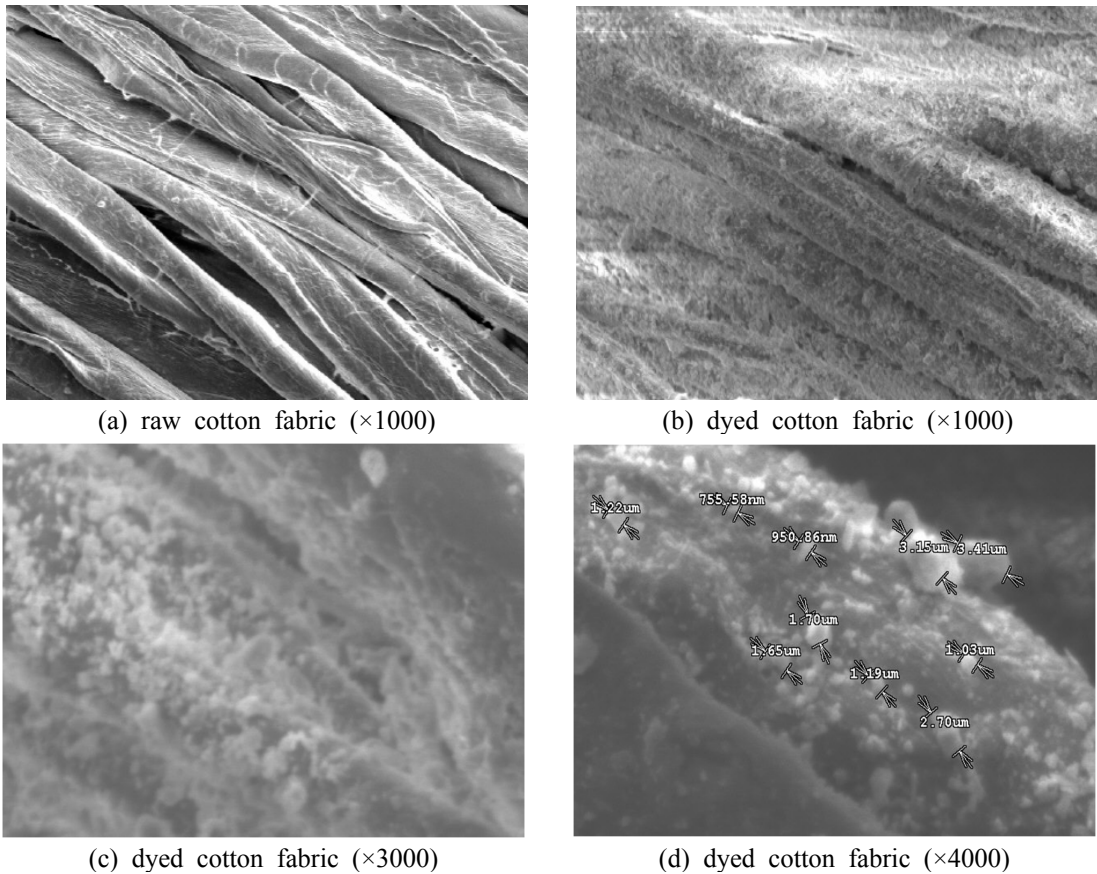
Fig. 4. SEM photographs of cotton fabrics dyed with Jeju scorja .
