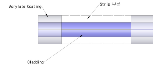
Fig. 6 Optical fiber stripped jacket.
