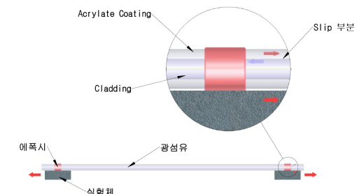
Fig. 5 Ordinary fixing method of fiber sensor.
