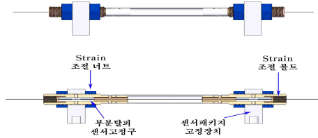
Fig. 8 Optical fiber sensor packages with stripped fiber fixture.
