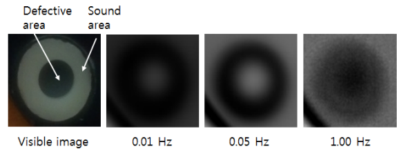
Fig. 5 Visible photo and the corresponding amplitude images of a specimen according to frequency conditions( t_d = 0.5 mm).
