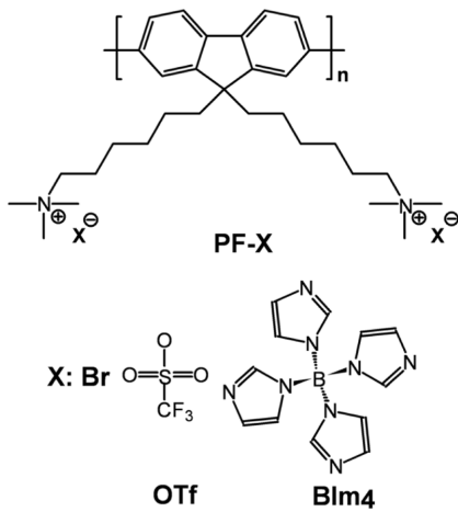
Figure 1. Chemical structures of conjugated polyelectrolytes.
