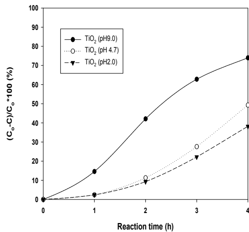
Fig. 6. Photocatalytic degradation of methylene blue under 30 W BLB lamp with 0.2 g of N-TiO 2 prepared at different pH.
