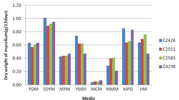
Fig. 4. Mycelial growth of C. pruinosa isolates in different liquid media at 25°C for 12 days. The data is the mean value of five replicates which is not statistically significant difference between replicates ( P < 0.05 ).
