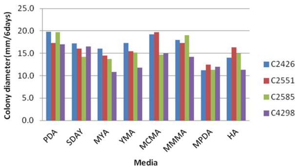
Fig. 2. Mycelial growth of C. pruinosa isolates on different solid media at 25°C for 6 days. The data is the mean value of five replicates which is not statistically significant difference between replicates ( P < 0.05 ).
