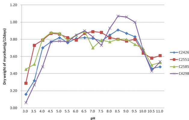
Fig. 5. Mycelial growth of C. pruinosa isolates on SDYM with different pH at 25°C for 12 days. The data is the mean value of five replicates which is not statistically significant difference between replicates ( P < 0.05 ).
