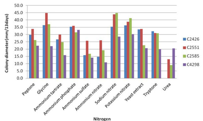
Fig. 7. Mycelial growth of C. pruinosa isolates on MPDA with each different nitrogen source at 25°C for 13 days. The data is the mean value of five replicates which is not statistically significant difference between replicates ( P < 0.05 ).
