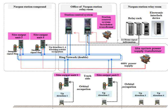
[Fig. 3] Configuration of Field Installation
