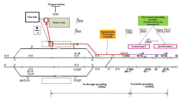
[Fig. 2] Schematic Diagram of Field Installation
