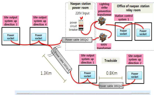
[Fig. 9] Power Line Configuration for Field Test
