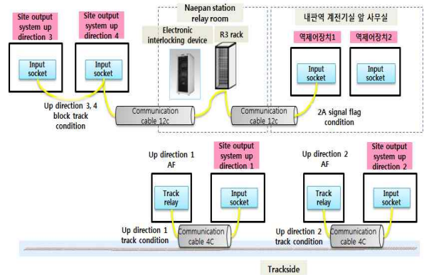
[Fig. 11] Wiring Diagram of Electronic Block System
