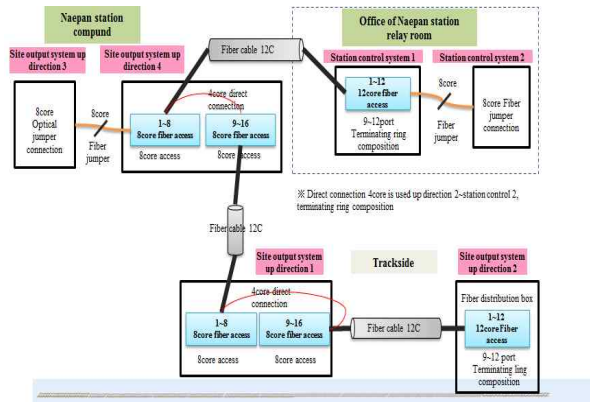
[Fig. 10] Optical Cable Configuration for Field Test
