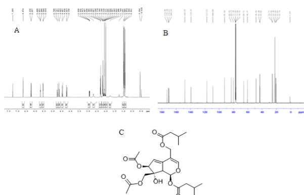
Figure 1. Isovaltrate Acetoxyhydrin (IA) and Its Nuclear Magnetic Resonance Spectra. (A) ^1\text{H} NMR of IA. (B) ^{13}\text{C} NMR of IA. ^1\text{H} NMR and ^{13}\text{C} NMR spectra were measured on Bruker DRX-400 NMR spectrometer operating at 400 MHz, and \text{CDCl}_3 was used as solvent. (C) Chemical structure of IA
