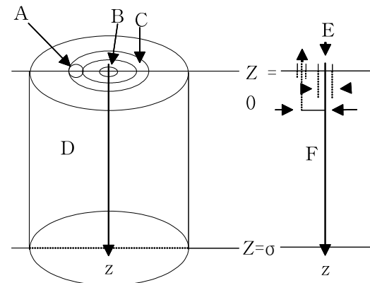
Fig. 1. Geometry to measure the reflected light as a function of the distance to an incident beam A: measuring area, B: source, C: detection ring, D: scattering volume, E: incident beam, F: scattering medium.
