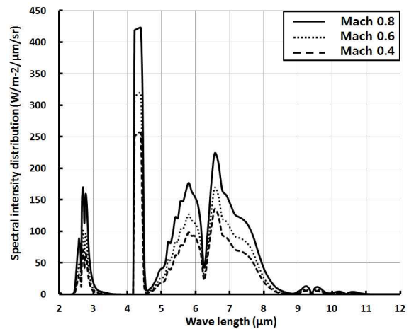
Fig. 14. Spectral intensity with wavelength (20,000 ft, angle 90°)
