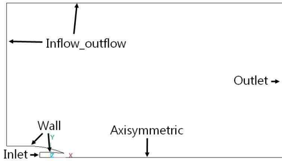
Fig. 5. Numerical boundary conditions (circular nozzle)
