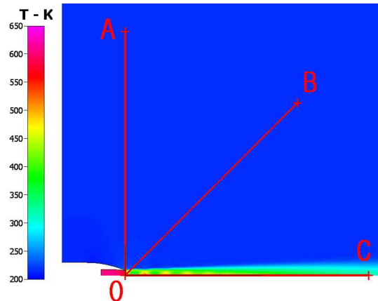
Fig. 11. The position of plume IR observation
