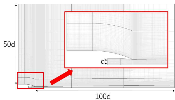
Fig. 4. Grids around nozzle
