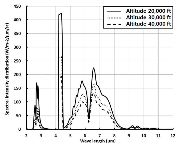
Fig. 15. Spectral intensity with wavelength (Mach 0.8, angle 90°)
