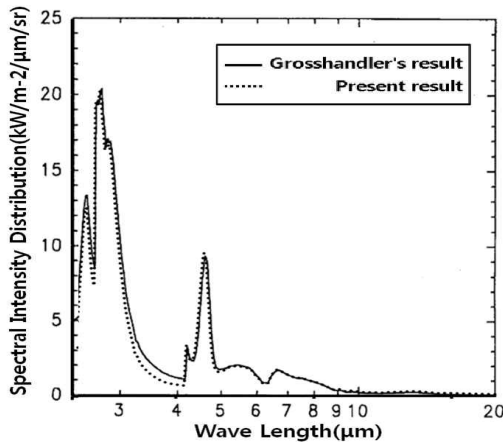
Fig. 8. Validation of the narrow band model
