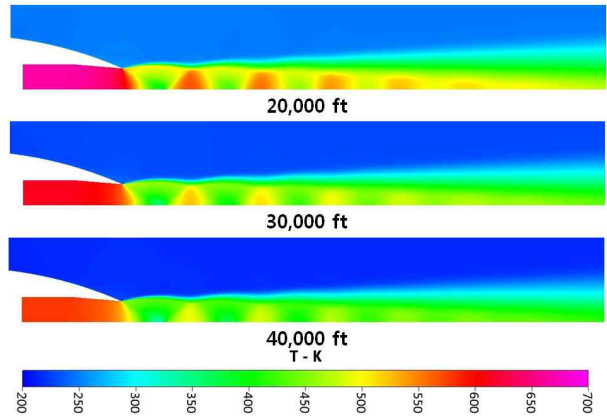
Fig. 10. Contours of temperature (Mach 0.8)
