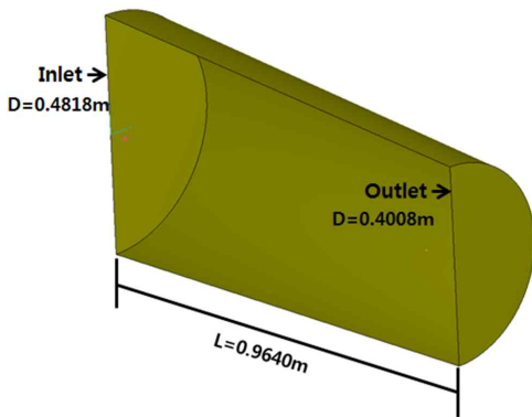
Fig. 3. Nozzle geometry
