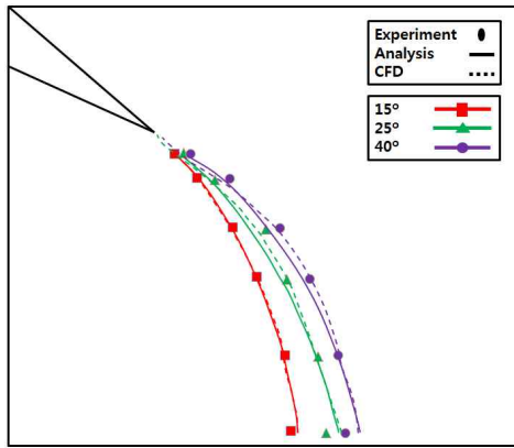
Fig. 7. Sonic lines for various nozzle angles (NPR 2.5)
