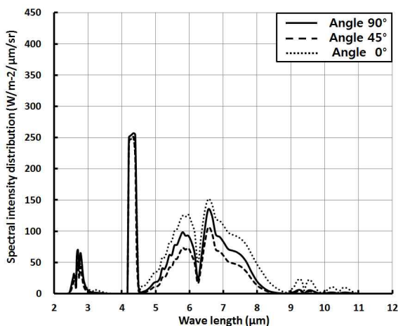
Fig. 12. Spectral intensity with wavelength (20,000 ft, Mach 0.4)
