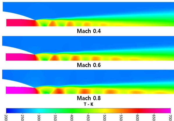
Fig. 9. Contours of temperature (20,000 ft)
