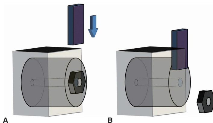
Fig. 2. Schematic presentation of shear bond test. A: the mounting specimen and loading, B: failure.
