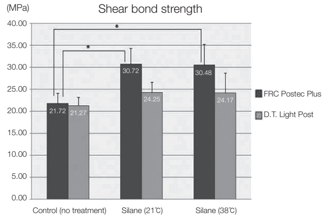
Fig. 3. Shear bond strength of the FRC Postec Plus and the D.T. Light Post as a function of the surface treatment. *: Mean values were significantly different by 1-way ANOVA ( P < .05 ).
