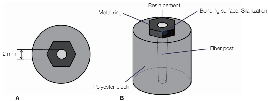
Fig. 1. Schematic drawing of specimen preparation for shear bond strength test. A: cross-sectional view for shear bond test, B: total view of mounted specimen.
