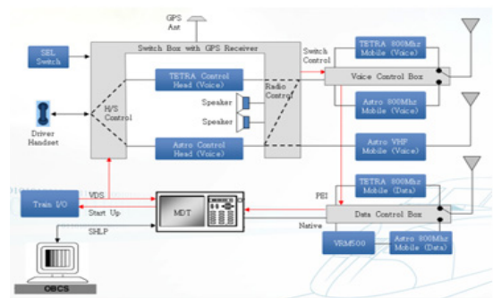
[Fig. 2] On-board System of KTX TRS
