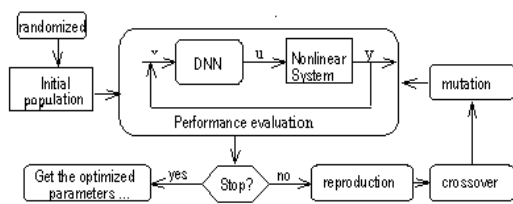
Fig.5 A functional block diagram showing the GA optimization process.
