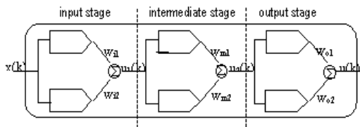
Fig4. the Dynamic Neural Network structure
