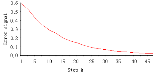
Fig.10 The Error Signal of DNN Using GA
