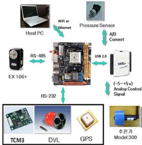
Figure 9: Block diagram for hardware system
