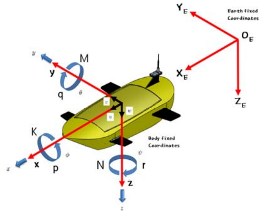
Figure 2: Coordinate system of Manta UUV
