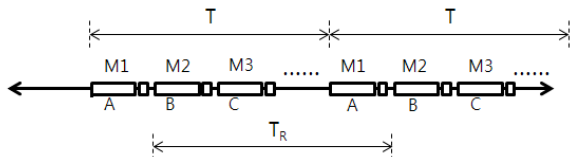
Fig. 3. Multi-Message Chain-Single Buffer
