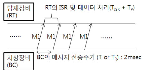
Fig. 6. Data Transfer Method of the current system
