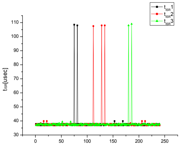
Fig. 8. Interrupt Service Routine Execution Time( t_{ISR} ) of current System
