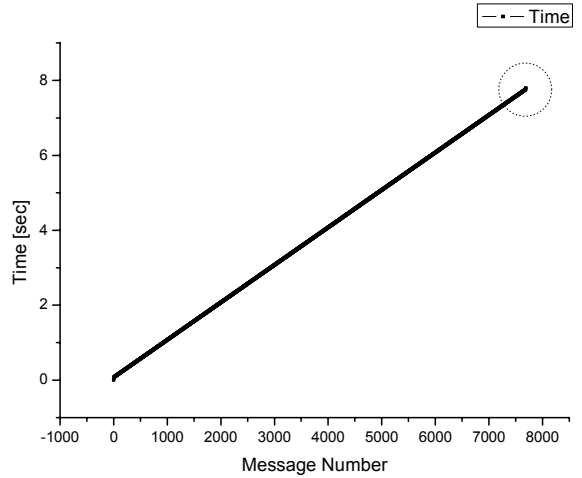
Fig. 12. Bus Monitor Result 1/2
