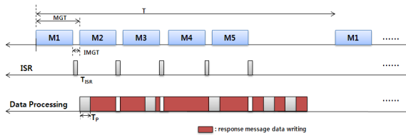
Fig. 10. Response Message Writing Time in Data processing of current System
