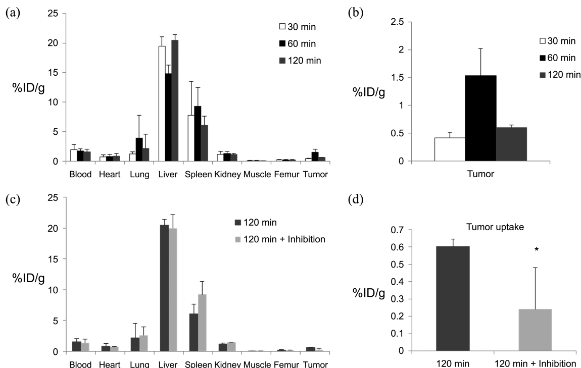
Figure 4. (a) Biodistribution of ^{68}\text{Ga} -NOTA-HT2-folate (3.7 MBq) in nude mice bearing KB cells at 30, 60, and 120 min after injection. (b) Tumor uptake at 30, 60, and 120 min after injection. (c) and (d) Tumor uptake and folic acid inhibition studies with the radioligand at 120 min after injection. Values represent mean %ID/g, and the error bars indicate SD ( n = 3 ). * P < 0.05
