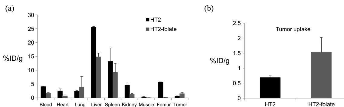
Figure 5. (a) Biodistribution of ^{68}\text{Ga} -NOTA-HT2-folate (gray) and ^{68}\text{Ga} -NOTA-HT2 (black) (3.7 MBq) in nude mice bearing KB cells at 1 h after radioligand injection via the tail vein. Values represent mean %ID/g and the error bars indicate SD (n = 3). (b) Tumor uptake (%ID/g) at 1 h after radioligand injection. * P < 0.05 .
