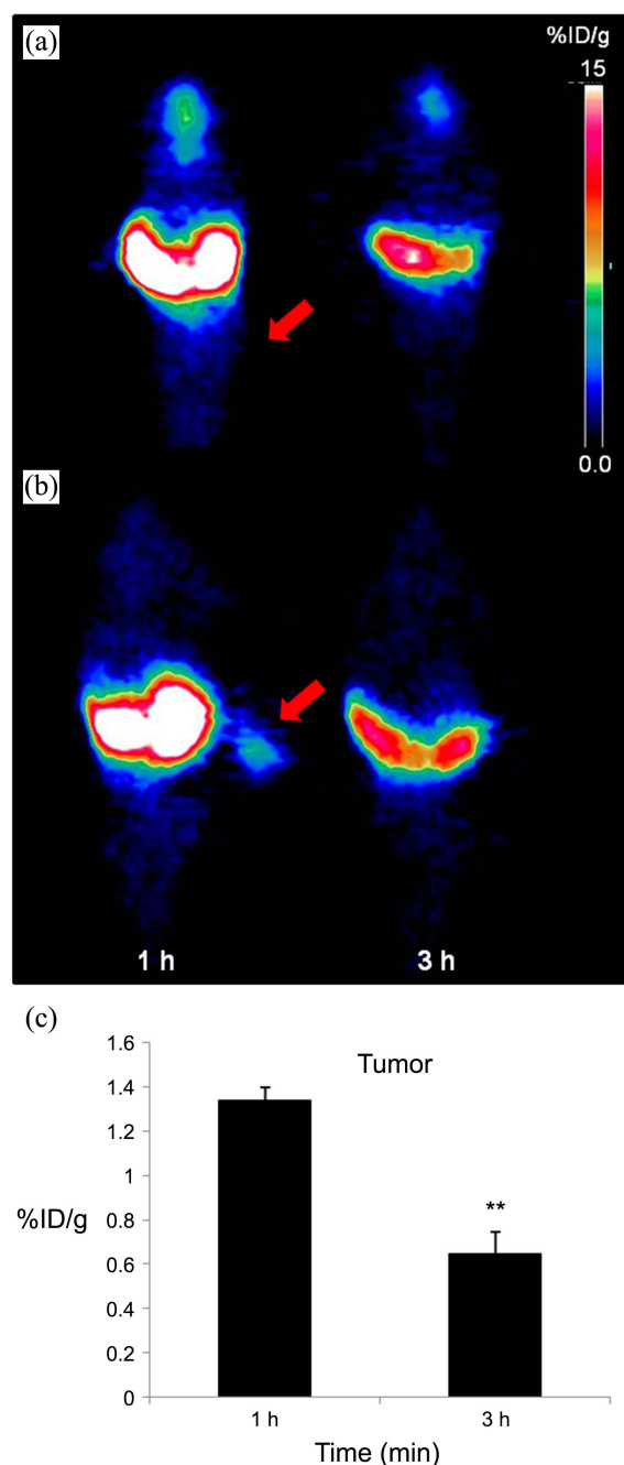
Figure 3. MicroPET images. Coronal microPET images of 68 Ga-NOTA-HT2 (a) and 68 Ga-NOTA-HT2-folate (7.4 MBq) (b) injected into mice bearing KB tumor cells at 1 and 3 h after injection. Arrows indicate the position of the KB tumor. The images are displayed at different values of %ID/g. (c) ROIs of the tumor with 68 Ga-NOTA-HT2-folate 1 and 3 h after injection. ** P < 0.01.
