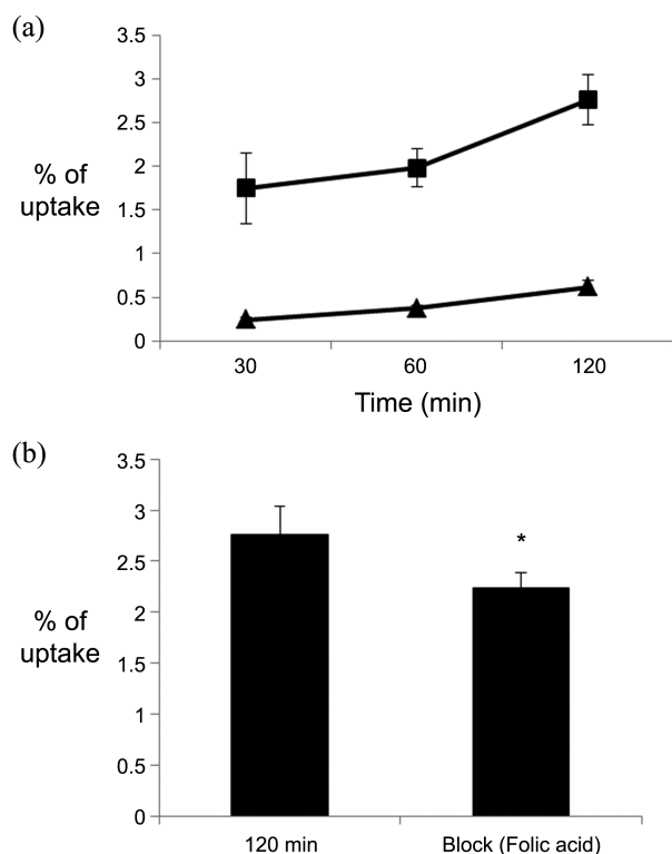
Figure 2. KB tumor cell uptake of 68 Ga-NOTA-HT2-folate and 68 Ga-NOTA-HT2 in vitro . (a) Tumor cell uptake (% of uptake) of the radioligand is shown as a function of time. ■: KB tumor cell uptake of 68 Ga-NOTA-HT2-folate; ▲: KB tumor cell uptake of 68 Ga-NOTA-HT2. (b) KB tumor cell uptake of 68 Ga-NOTA-HT2-folate with and without 100 μg folic acid at 2 h incubation. * P < 0.05.
