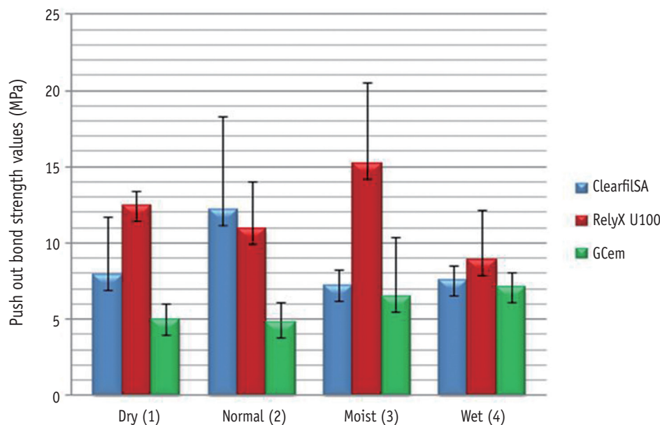
Figure 1. Push-out bond strengths (MPa) of self adhesive cements with respect to the experimental moisture conditions.
