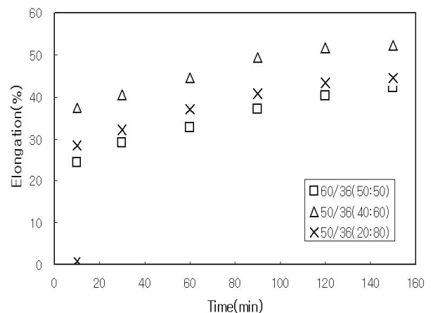
Figure 7. Elongation of yarns against treated time at NaOH 20%, 50°C.
