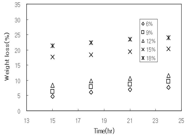
Figure 10. Weight loss of woven against treated time at various NaOH solution at 35°C, 50d/36(N/P 20:80).
