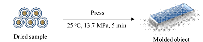
Scheme 1. Preparation procedures for synthesis of core/PBA/PS double shell nanoparticles and baroplastic process at room temperature.
