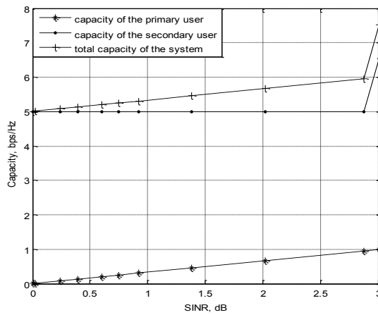
Fig. 7. Relation between capacity and SINR of PU
