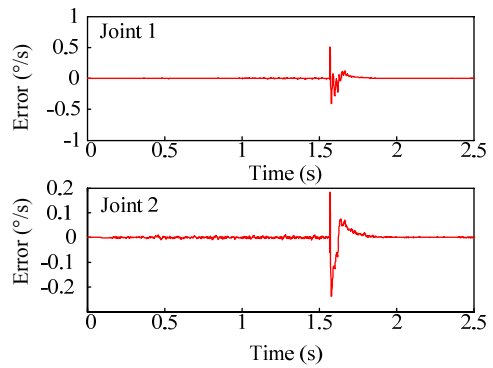
Fig. 6. Velocity error upon dynamic collision
