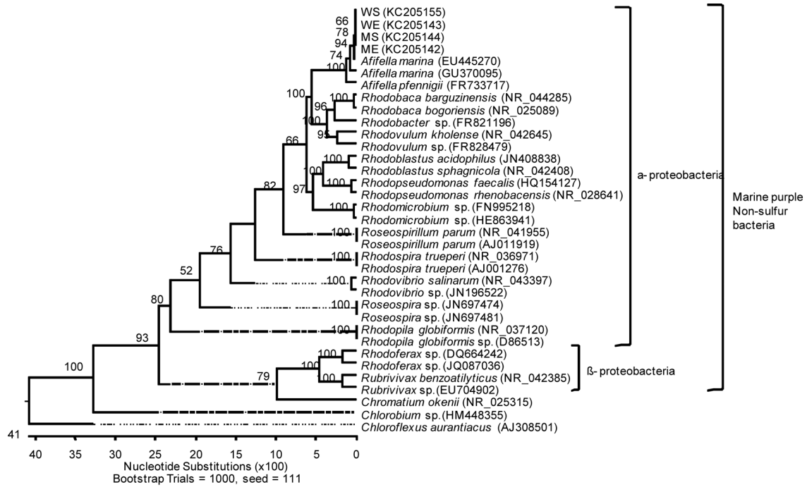
Fig. 1. Phylogenetic tree of 16S rRNA gene sequences of isolates and strains from representative marine PNSB genera. The tree is rooted with Chloroflexus aurantiacus strain DSM 637T (AJ308501), Chlorobium sp. (HM448355), and Chromatium okenii (NR_025315) as an out-group. Bootstrap values are given at branch points.
