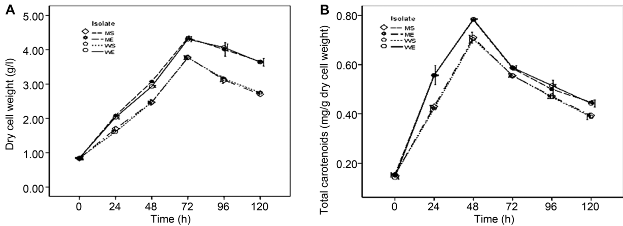
Fig. 2. Changes in (A) dry cell weight (g/l) and (B) total carotenoids (mg/g) of isolates grown under anaerobic-light (2.5 klx) conditions at 30 \pm 2^\circ\text{C} , over a period of 120 h.
