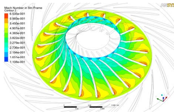
Figure 5: Distribution of Mach number at the rotor
