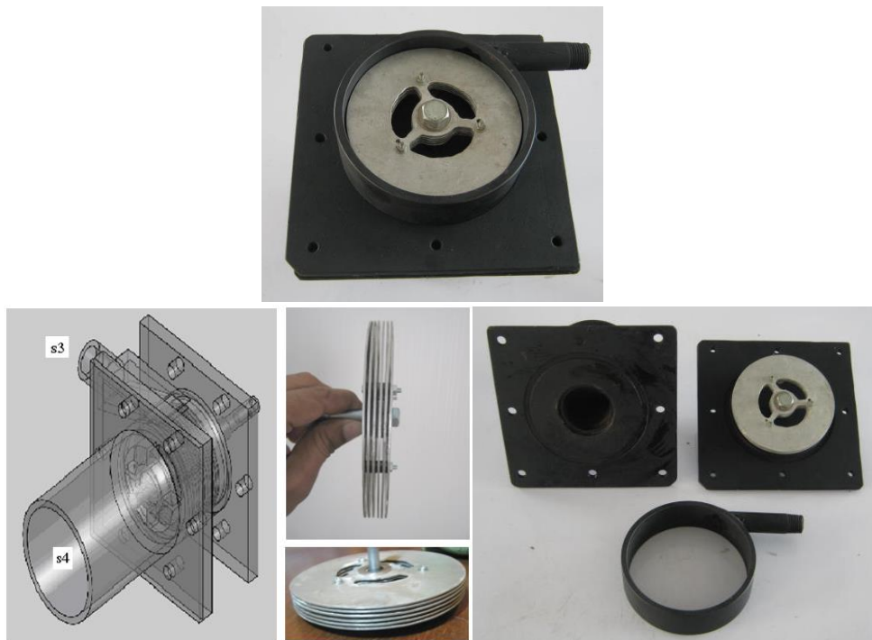
Figure 3. Tasla turbine plate of the first size.
