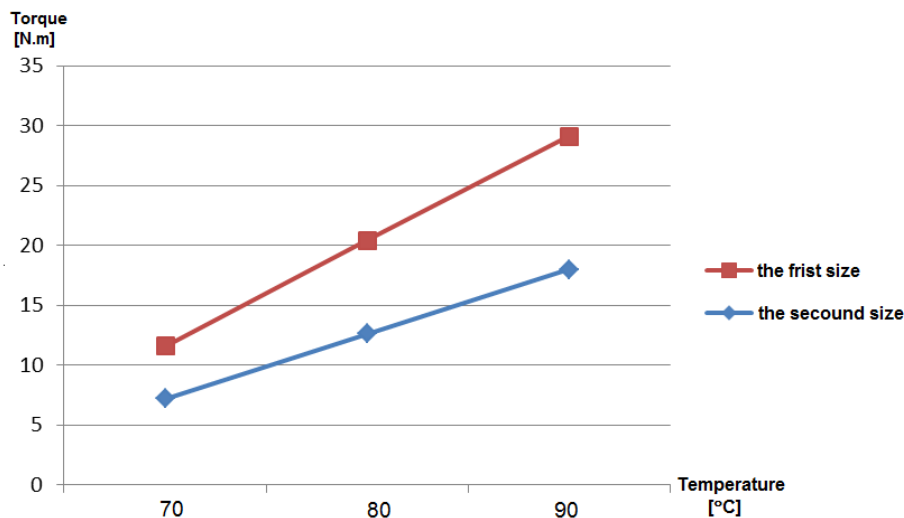
Figure 6. Result of comparison of two-size Tesla Turbines
