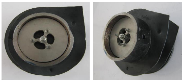
Figure 4. Tasla turbine plate of the Second size.
