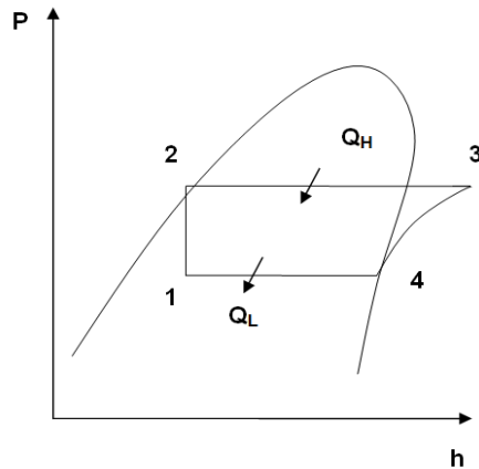
Figure 1. P-h diagram of the Rankine cycle
