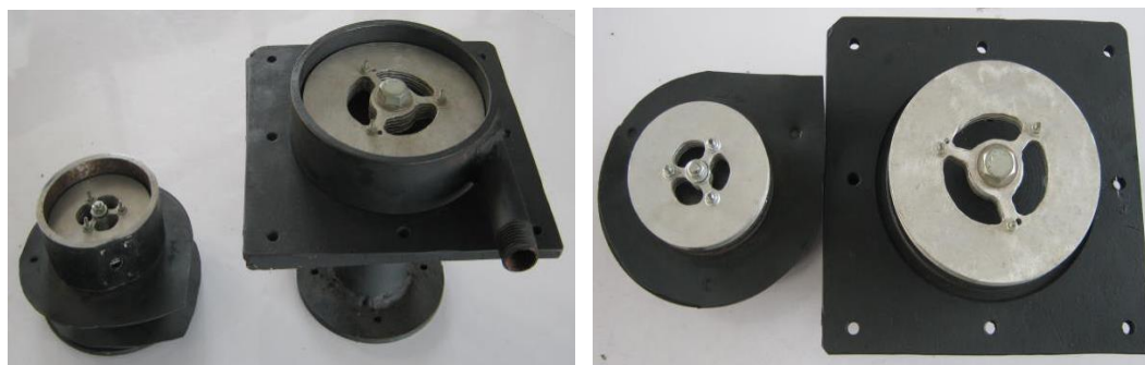
Figure 5. Comparison of two-size Tesla Turbines.
