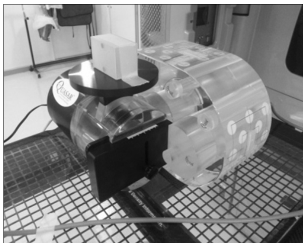
Fig. 1. Experimental setup of the programmable respiratory motion phantom. The insert containing the film or ion chamber moves in the inferior-superior direction, and the top platform moves in the anterior-posterior direction for the RPM block.
