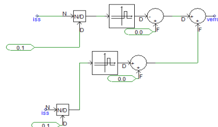
[Fig. 9] Control modelling of BESS
