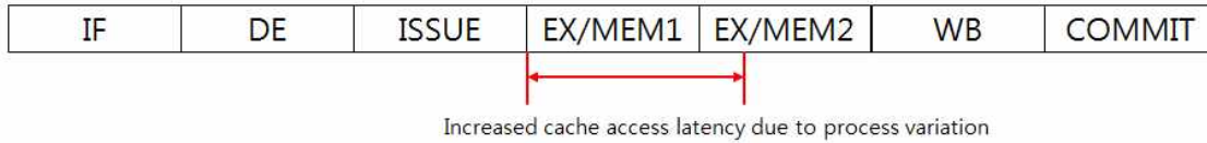
(b) In the case of saving a chip from an yield loss by employing variable latency L1 data cache
