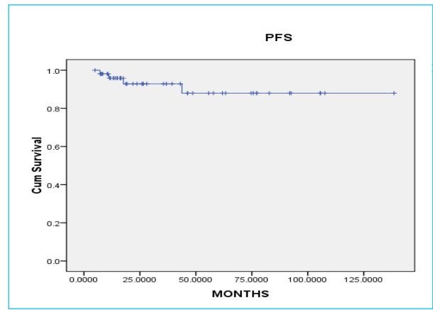
Figure 1. Cumulative PFS
