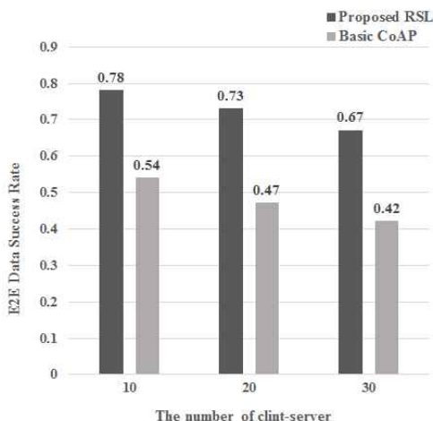
Fig. 13 Average end-to-end data transmission success rate in the sleep mode of node environment
