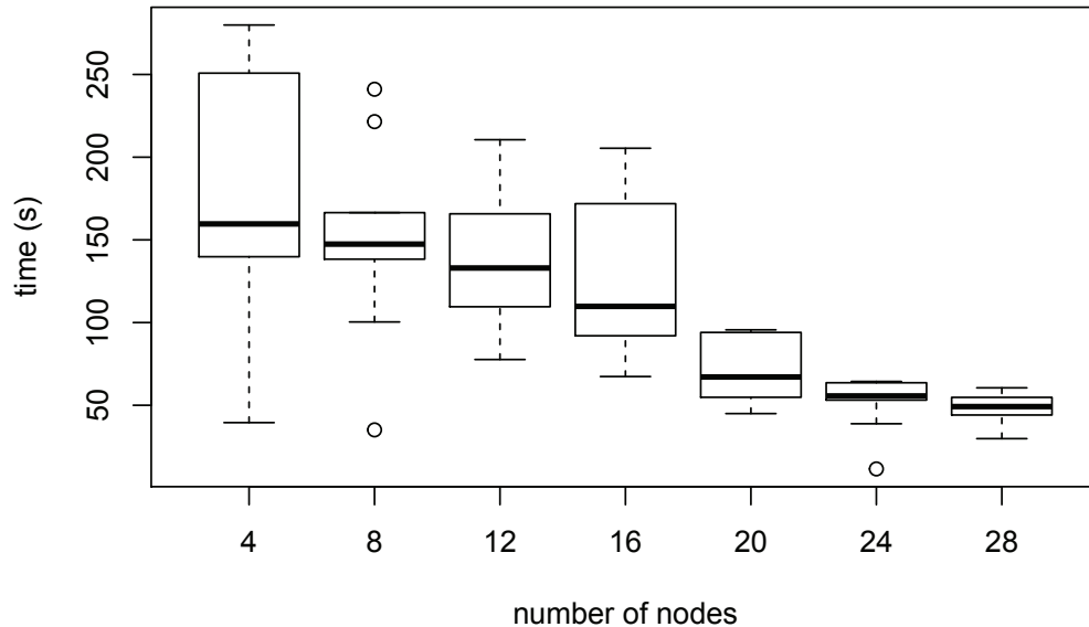
Figure 7.1. Boxplot of time elapsed for the K -means benchmark experiment. One million 100-dimensional data points were clustered into 100 clusters for 300 iterations. The experiment was performed with 4, 8, 12, 16, 20, 24, 28 nodes, with 10 repetitions each.
