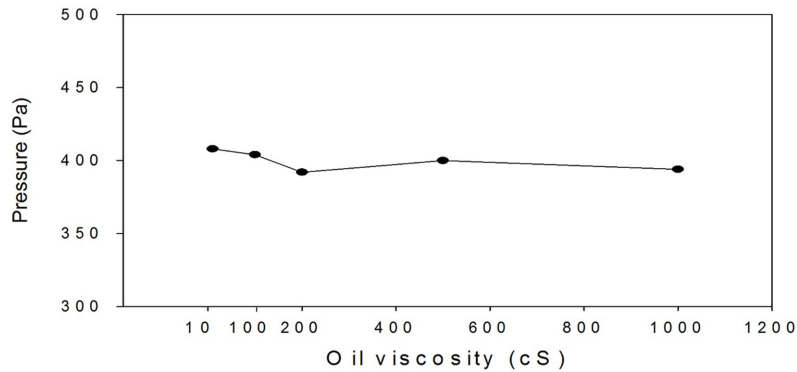
Fig. 3. Open pressures of the degassing valve having applied the silicon oil with 10, 100, 200, 500, 1000 cS of viscosity to 0.8 mm thick rubber disk.
