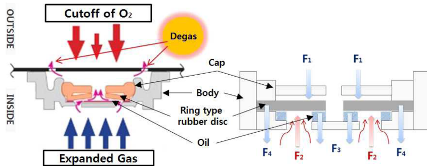
Fig. 1. Structure and degassing mechanism of the one way valve with ring type rubber disk 4) : (F 1 ) the outer atmospheric pressure; (F 2 ) the inner pressure; (F 3 ) the oil capillary adhesion; (F 4 ) the rubber elastic strength.
