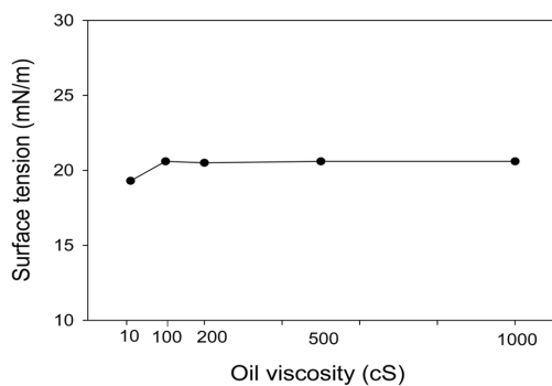
Fig. 4. Surface tensions of the silicon oil with 10, 100, 200, 500, 1000 cS of viscosity.
