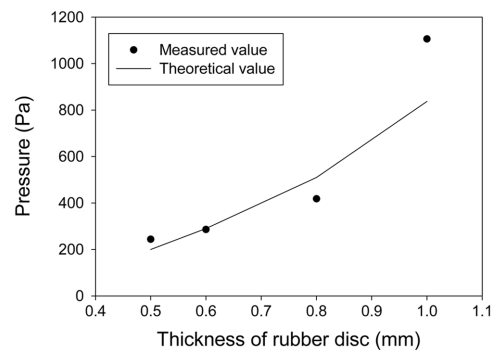
Fig. 5. Theoretical degassing pressure-disc thickness curve and experimental results for the degassing valves.
