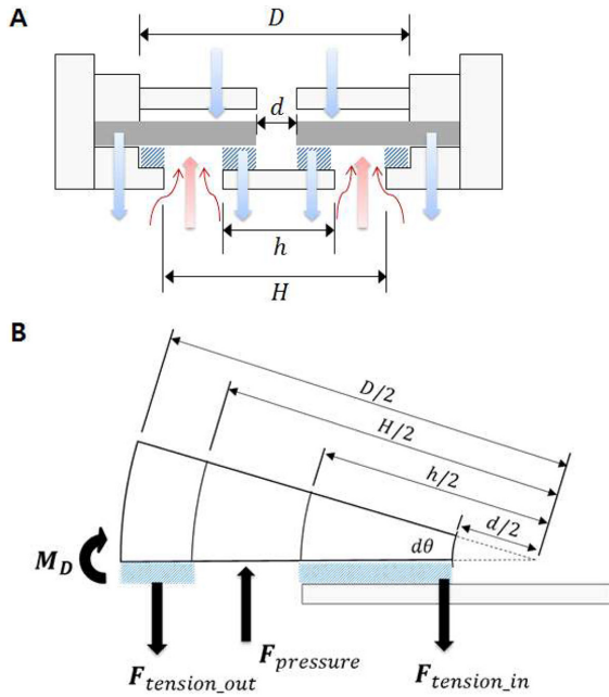
Fig. 2. Free body diagrams for the mechanical analysis of the degassing valve by the inner pressure, the oil capillary adhesion and the rubber elastic strength: overview (A); partial view (B).
