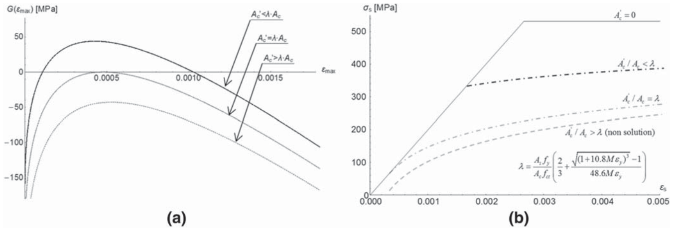
Fig. 3 Parameters of RC section: f_y = 530 MPa, f_{ct} = 4.50 MPa, A_s = 50.27 mm 2 (1 Ø 8), A_c = 9025 mm 2 : a Function G[\varepsilon_{max}] for different values of A'_c ; the equation G[\varepsilon_{max}] = 0 has no positive real solutions when A'_c/A_c is greater than the limit value \lambda . b Effect of tension stiffening area over the embedded steel behavior model.
