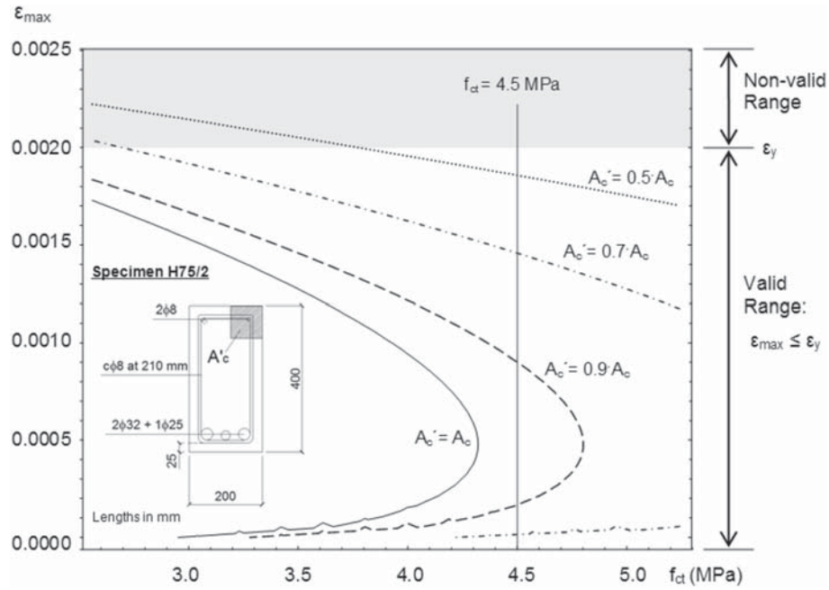
Fig. 2 Specimen H 75/2 (Cladera Bohigas 2002): solvability graphical analysis for apparent yield strain ( \varepsilon_{max} ) in the top longitudinal reinforcement.
