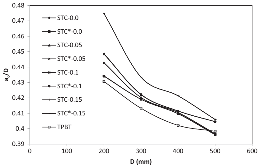
Fig. 6 Comparison in the values of a_c/D for STC obtained using the previous method (Kumar and Pandey 2012) and the present revised method.
