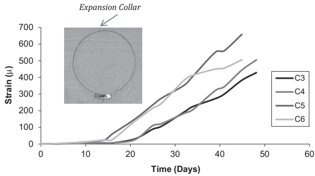
Fig. 9 Variation of the circumferential expansion with time for all specimens as measured with mechanical expansion collar.
