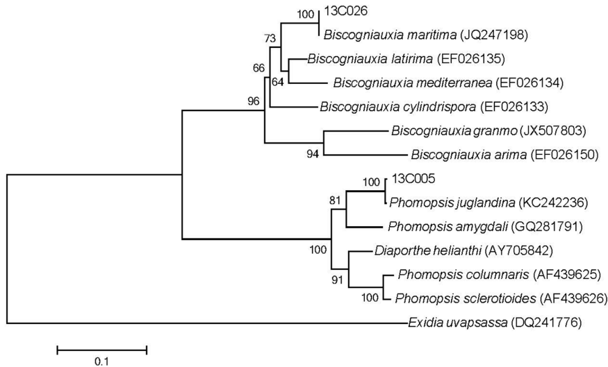
Fig. 2. Neighbor-joining tree of Biscogniauxia maritime , Phomopsis juglandina isolates based on internal transcribed spacer and 5.8S rDNA region. This region was used to confirm the topological appropriation of the isolates. Exidia uvapassa was used as an outgroup.
