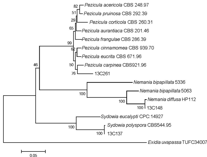
Fig. 1. Neighbor-joining tree of Sydowia polyspora , Nemaniam diffusa , Pezicula carpineae isolates based on a combined alignment of internal transcribed spacer and large subunit rDNA sequences. Exidia uvapassa was used as an outgroup.
