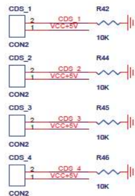
Fig. 10. Circuit design for CDS sensor
