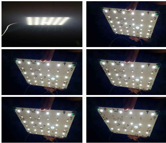
Fig. 14. Dimming Control by Visual Response
