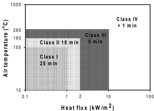
Fig. 6. Graphical representation of the recommendations for thermal classes of fire fighter environments [8]
